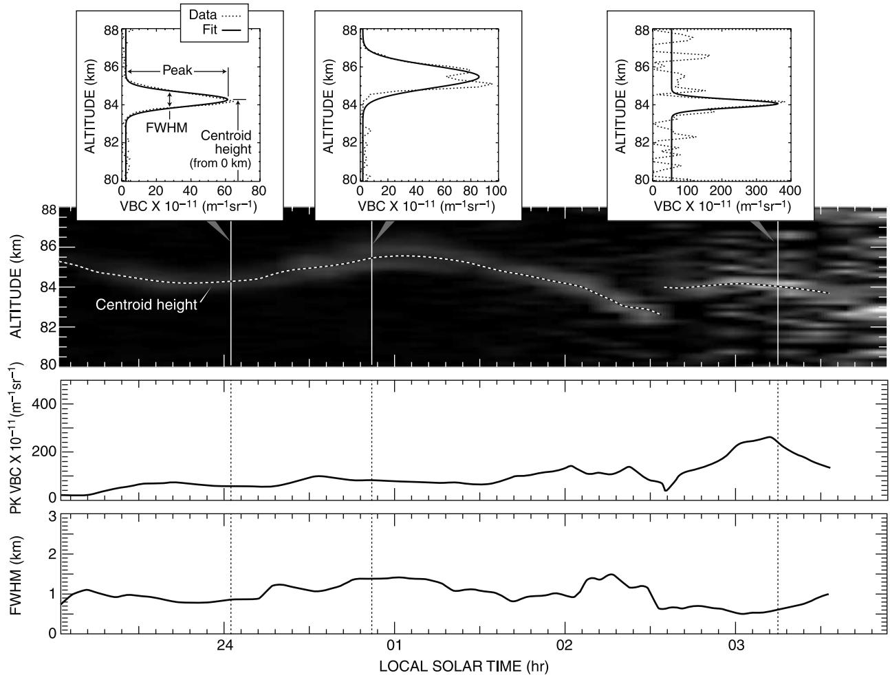
Figure 2. Lidar observations of an NLC on 8 August 1996 and select profiles to illustrate the Gaussian fit procedure to derive the cloud centroid height, FWHM, and VBC.
