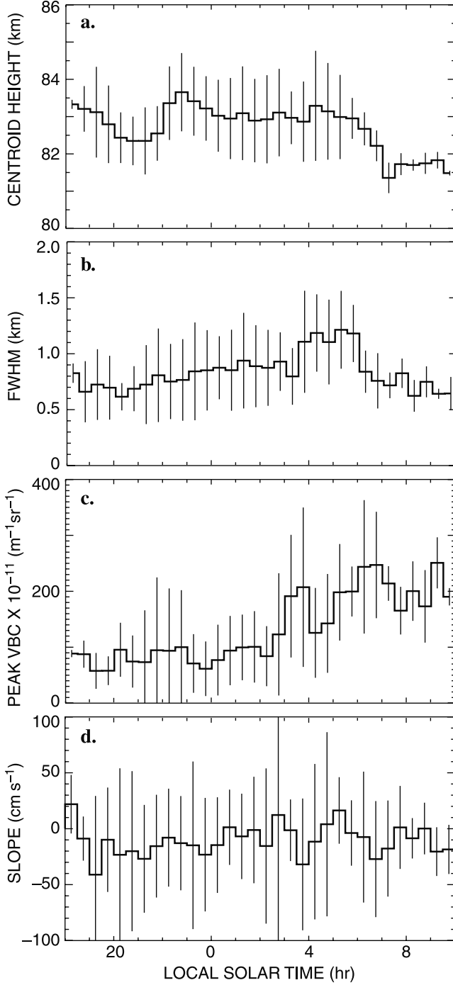
Figure 5. Derived NLC parameters of (a) centroid height, (b) FWHM, (c) VBC, and (d) time rate of change in centroid height averaged into 30-min local time bins. The error bars represent the geophysical variability in the data.
