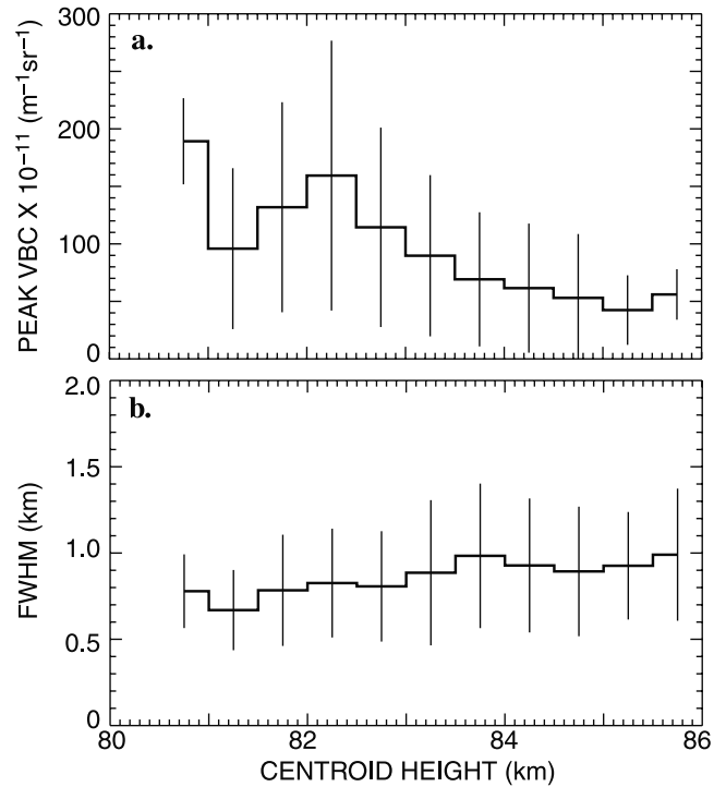
Figure 7. (a) VBC and (b) FWHM values organized into 0.5 km centroid height bins and averaged. The vertical lines represent the standard deviation resulting from the averaging.
